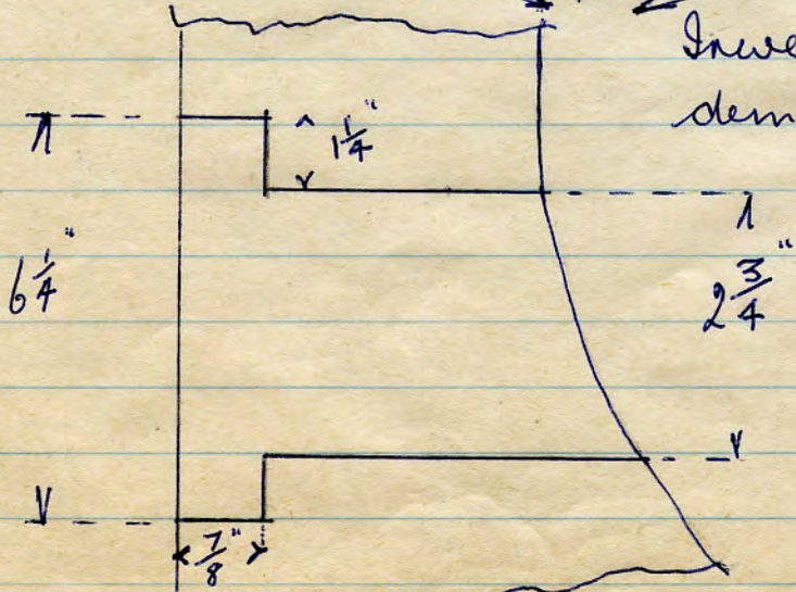
Section through bolt hole.
